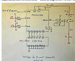
1. This circuit, based on a PIC microcontroller with a few added components, converts a sensor base voltage into a 4- to 20-mA current loop. Shown is the circuit as originally designed in a whiteboard.
